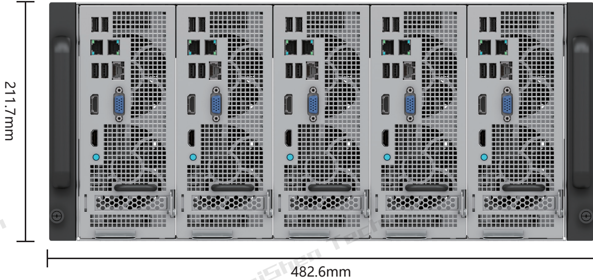
Front View (Dimensions)
