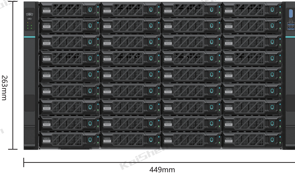
Front View (Dimensions)
